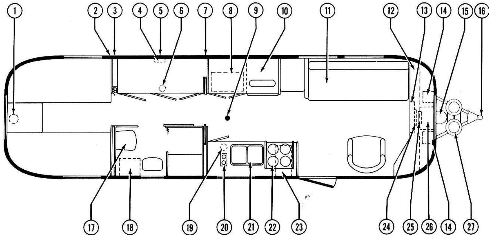
Floor Plan - Center Bath Twin
