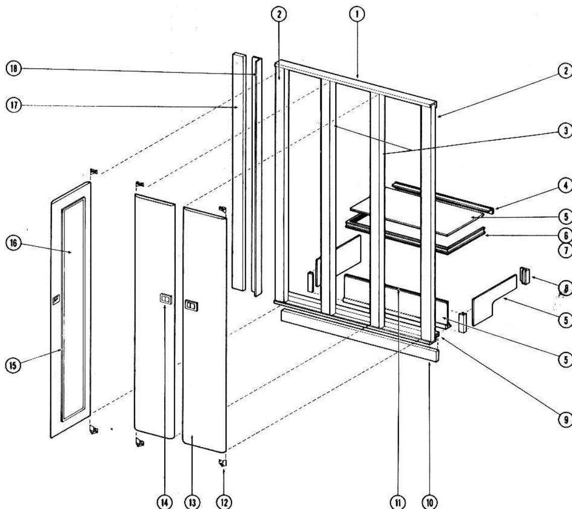
Triple Wardrobe Assembly 50"- 67½"
