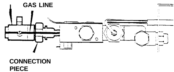
SHUT-OFF VALVE
